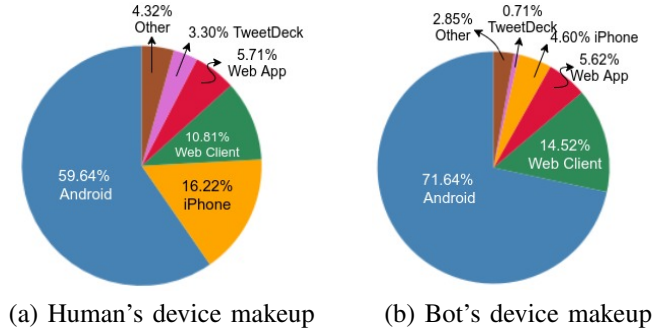
Figure 2: Device makeup for humans and bot accounts. Both groups have largest proportion of traffic coming from Android phones, which is an indicator of that bots are actually humans.
