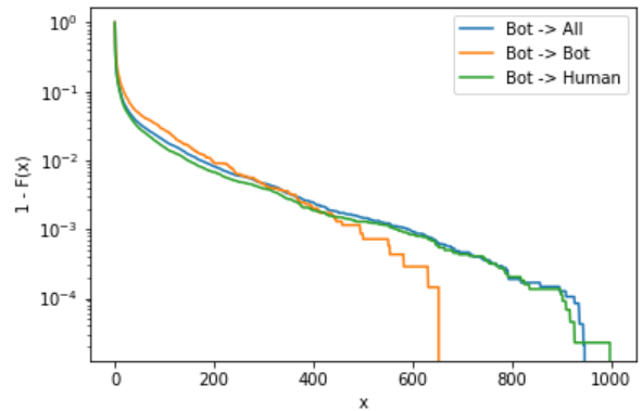
(a) CCDF of Retweets done by bots
