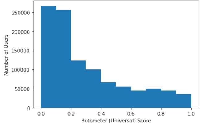
Figure 1: Distribution of Botometer score for 1,046,260 users
