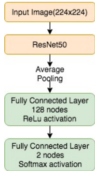
Figure 1: Proposed Model. We used 3-fold Cross-validation and found that 128 nodes in the dense layer gives best Cross-validation accuracy.
